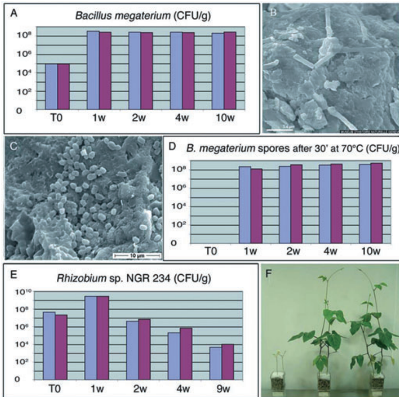
Fig. 4. Survival of Bacillus megaterium B13 and Rhizobium sp. NGR234 on dry sand. A, D and E. Vertical axes – number of bacteria in cfu g -1 sand; horizontal axes – time in weeks (w). Blue and burgundy colours represent two separate replicates. A. Numbers of B. megaterium as a function of time. B. B. megaterium -like cells on the surfaces of a historic sand grain (vial # 2987a). C and D. After 1 week of desiccation, spores dominate on dry sand (C – SEM, and D – numbers after heating to 70°C and plating out). E and F. Non-spore-forming Gram-negative bacteria (here Rhizobium sp. NGR234) survive extended periods of desiccation without losing their capacity to form functional nitrogen-fixing symbioses with legumes. E. Numbers of rhizobia on the sand grains. F. Vigna unguiculata inoculated with wild-type NGR234 (centre), and NGR234 taken from sand grains held for 9 weeks at 20% relative humidity (pot at left – non-inoculated control).
