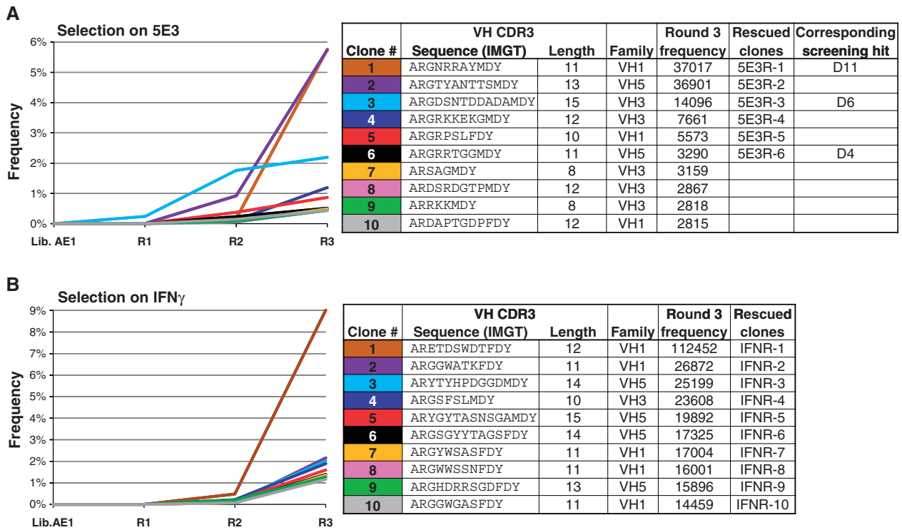
Figure 4. Frequency and evolution of top 10 sequences. Frequency of the 10 VH_{CDR3} sequences that were the most abundant after the third selection round against 5E3 (A) and against hIFN \gamma . (B) Amino acid sequence, length of the VH_{CDR3} according to the IMGT nomenclature and VH family are shown. Sequences that were also identified during screening by ELISA as well as clones that were rescued based on their VH_{CDR3} sequence and frequency are indicated.
