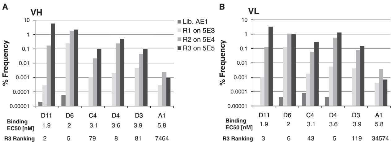
Figure 5. Frequency and evolution of CDR3 sequences identified by classical binding screening against the target 5E3. Frequency evolution of VH_{FR4-CDR3-FR3} (A) and VL_{CDR3-FR4} (B) sequences corresponding to six scFv binding specifically to the monoclonal 5E3. The EC 50 for binding of the soluble scFv to the target in ELISA and the frequency ranking after the third round of selection are indicated below each clone.
